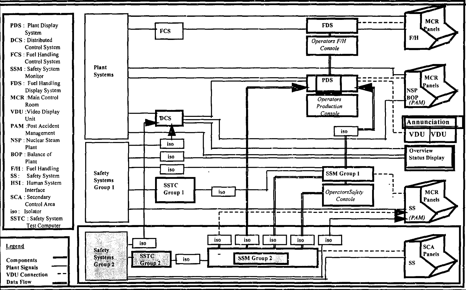
Figure 1: CANDU 9 Control Centre Functional Organization
